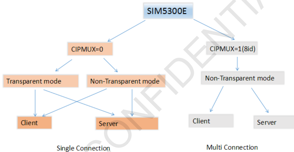
Figure1: SIM5300E TCPIP Structure
