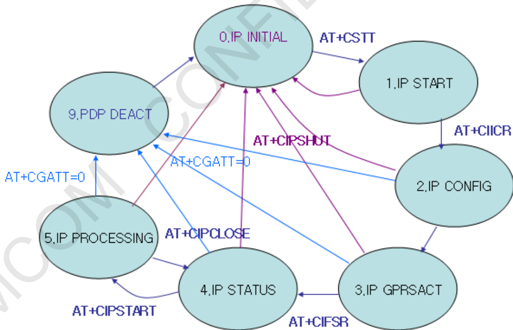
Figure2: GPRS States Diagram for single connection
